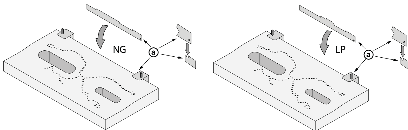
Figure 1: Deflector Replacement
